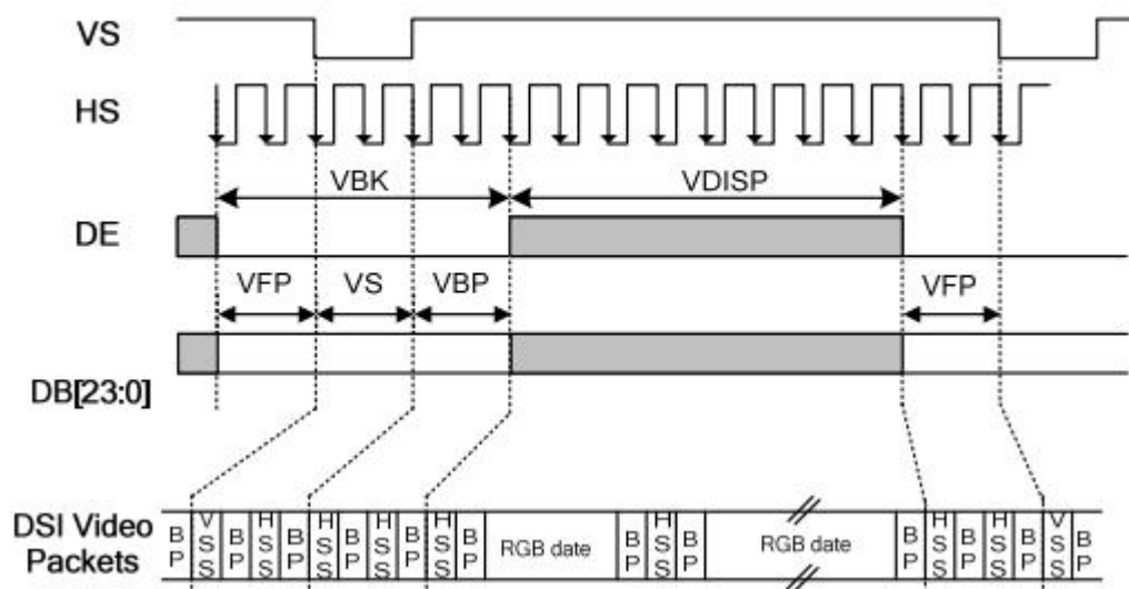
Vertical Timings for DPI I/F
