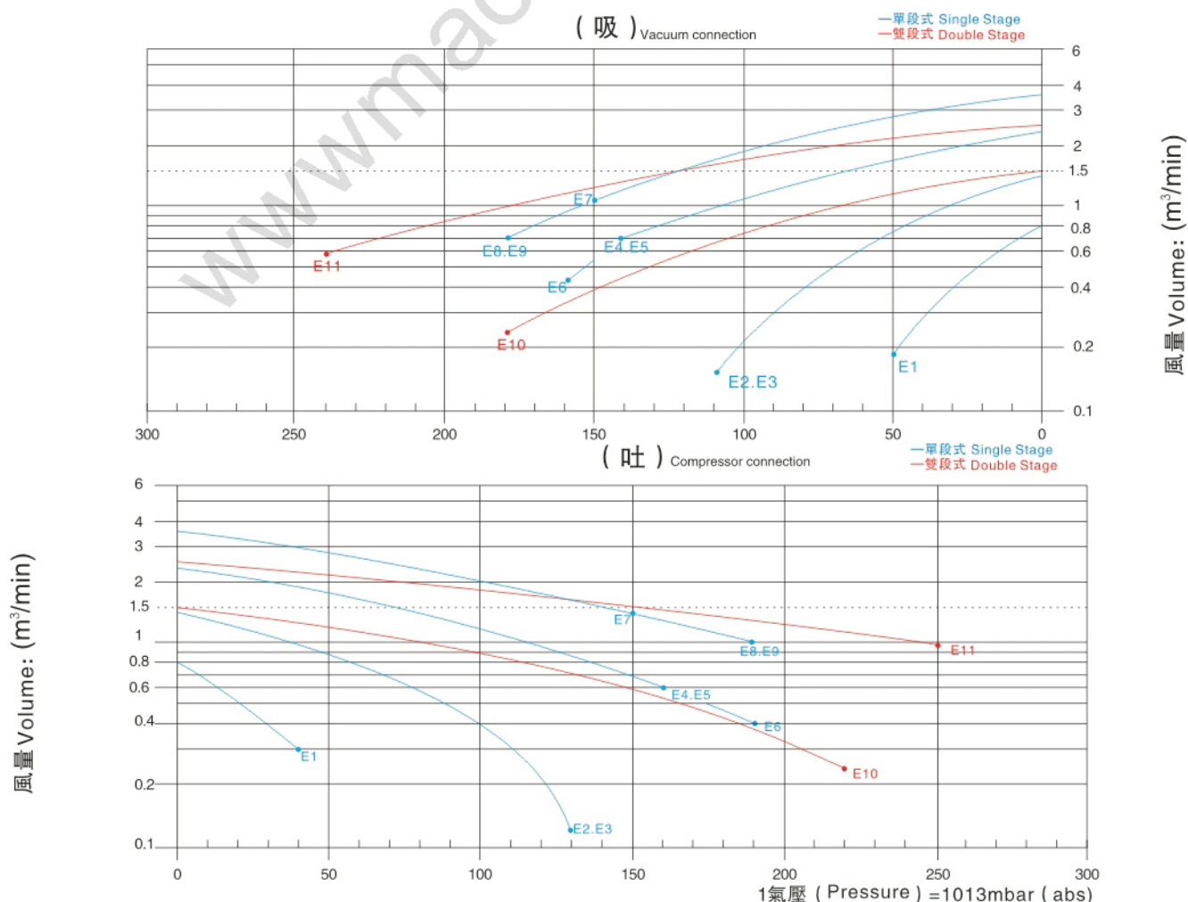
單相馬達, 50HZ吸/吐曲線圖 Single-phase motor, 50Hz handling curve diagram
