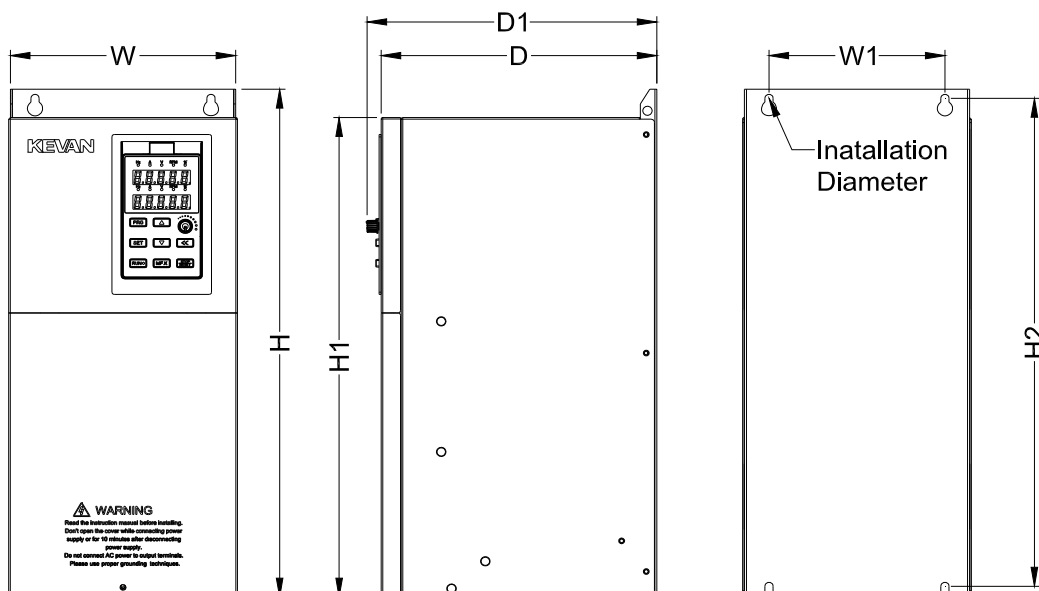
KV600 30G-400G Product dimensions
