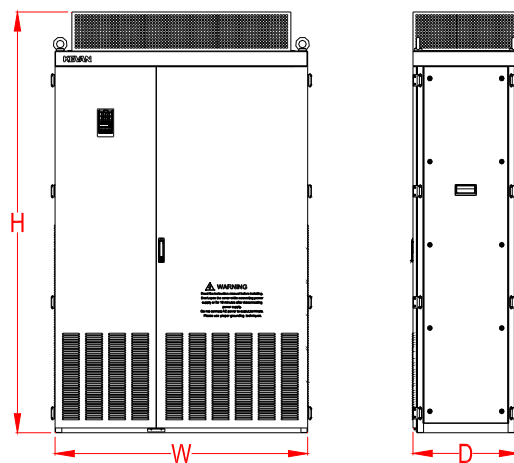
KV600 710G-900G Product dimensions
