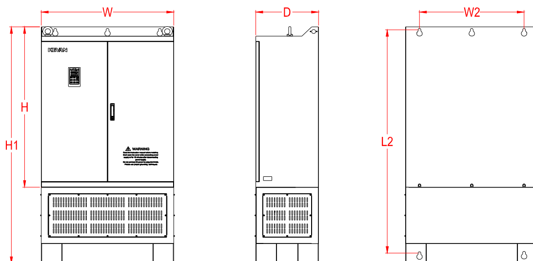
KV600 450G-630G Product dimensions
