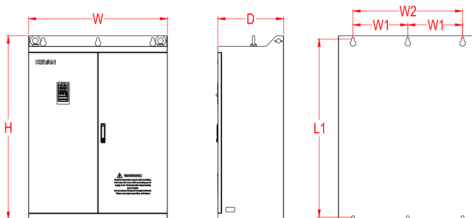
KV600 450G-630G Product dimensions
