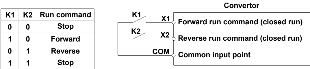
Schematic diagram of two-wire control 1
