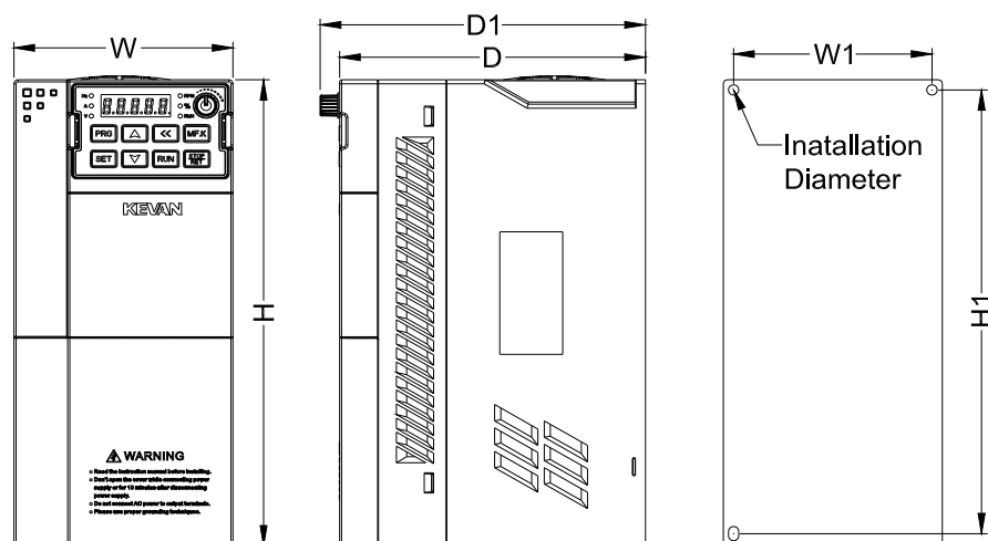
KV600 0.75G-22G Product dimensions
