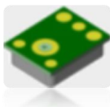
SMZ0603-06 3.76*2.95*1.1(mm) Sensitivity: -38\pm 1\text{dB/V} SNR: 64 dBA
