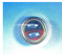
BY4015BOGB-C2 \Phi 4.0 \times 1.5 ( mm ) Sensitivity:-32 \pm 3dB SNR: 65dBA
